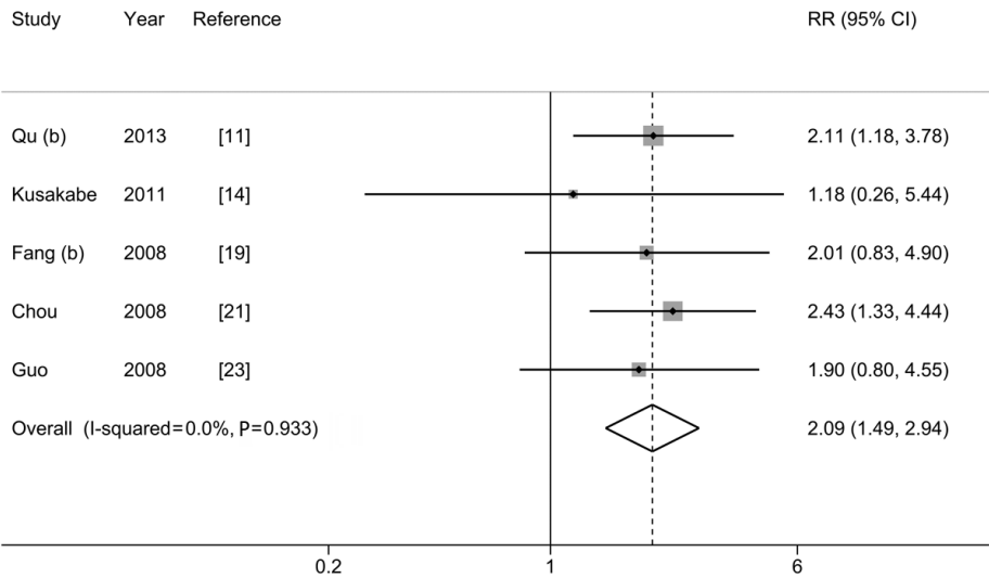
Figure 4 Results from meta-analysis of association between T1753V and hepatocellular carcinoma risk.
