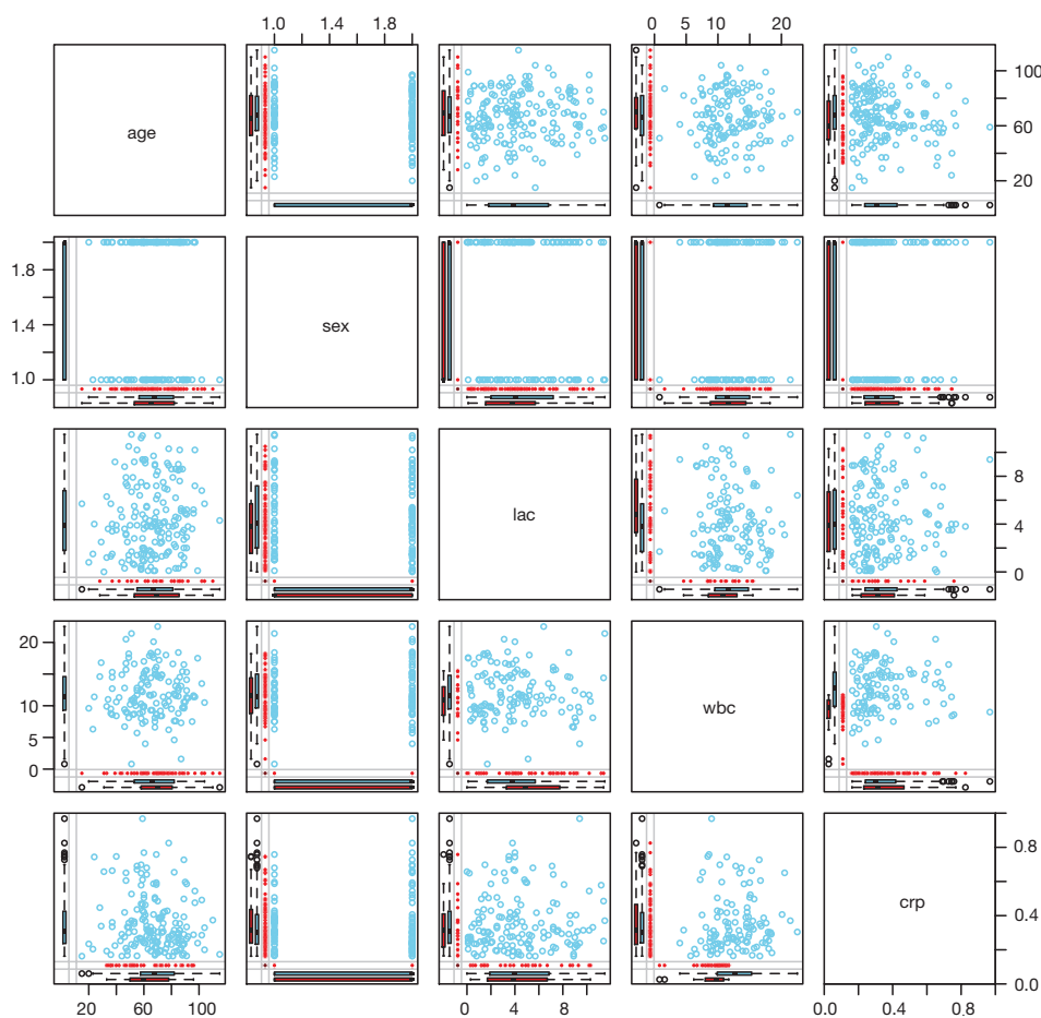
Figure 5 Scatterplot matrix with information about missing values in the plot margins of each panel.
