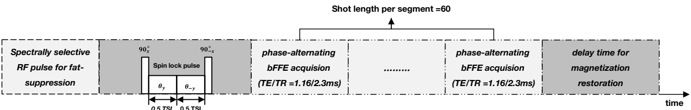
Figure 2 Diagram of the spin-lock balanced fast field echo (bFFE) imaging sequence for T1rho image (sequence 2). TSL = time of spin-lock pulse. The rotary-echo spin-lock pulse modified with Dixon method was used for T1rho preparation (13).
