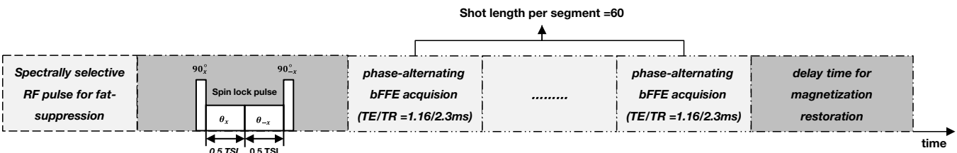
Figure 1 Diagram of the spin-lock balanced fast field echo (bFFE) imaging sequence for T1rho image (sequence 1). TSL = time of spin-lock pulse. The rotary-echo spin-lock pulse method was used for T1rho preparation.
