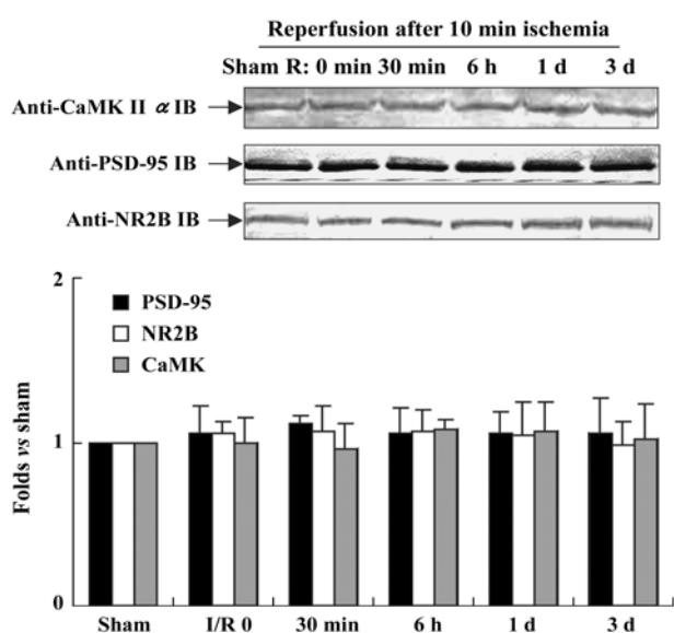
Fig 3. Immunoblotting analysis of the total protein levels of PSD-95, CaMKII \alpha , and NR2B during 0, 30 min, 6 h, 1 d, and 3 d reperfusion after 10 min ischemia. R, reperfusion, n=3 . Mean \pm SD.
