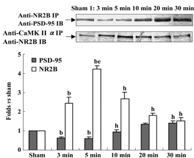
Fig 1. The interaction of PSD-95 with NR2B (upper panel) and CaMKII \alpha with NR2B (bottom panel) after 3, 5, 10, 20, and 30 min ischemia. I, ischemia. n=3 . Mean \pm SD. b P < 0.05 vs sham operation, c P < 0.05 vs 3 min ischemia, h P < 0.05 vs 5 min ischemia (ANOVA followed by LSD).
