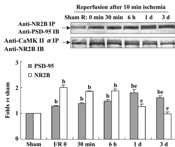
Fig 2. The interaction of PSD-95 and CaMKII \alpha with NR2B during 0, 30 min, 6 h, 1 d, and 3 d reperfusion after 10 min ischemia. R, reperfusion. n=3 . Mean \pm SD. b P < 0.05 vs sham operation, e P < 0.05 vs 10 min/R0 (ANOVA followed by LSD).
