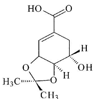
Structural formula of 3,4-oxo-isopropylidene-shikimic acid (ISA)
