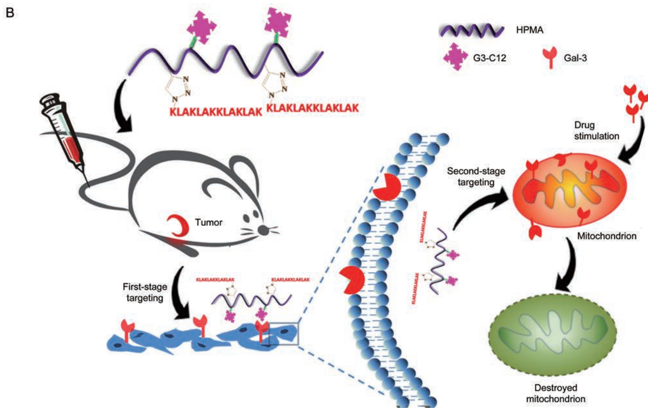
Scheme 1. (A) Synthesis route of G3-C12-HPMA-KLA conjugates. (B) Illustration of G3-C12-HPMA-KLA conjugates with sequential dual-targeting functionality from tumor cell surface to intracellular mitochondria.
