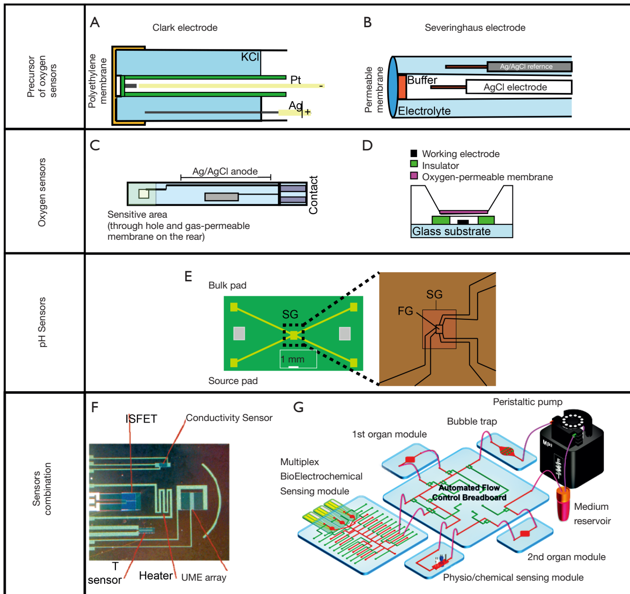
Figure 8 Precursor oxygen electrodes. (A) Cross-section of a Clark electrode containing 2 mm diameter platinum cathode; (B) the miniaturized Severinghaus needle oxygen electrode (123); (C) example to oxygen sensors; structure of a miniature oxygen electrode with glass substrate on which the cathode and anode patterns are formed (124); (D) cross-section of a miniature Clark oxygen sensor integrated with a container (125); (E) the reproduction of the sensor with zoom in view of the SG area and the schematic of the fluidic tester on top of the sensor (126); (F) full system integration: chip with integrated sensor for T measurement, pH (ISFET), dissolved oxygen concentration (UMEA) and the viable mass concentration (impedance sensor) (127) and (G) schematic of a full system where the multiorgan-on-a-chip platform was encased in incubator, and of automated pneumatic valve controller, electronics for operating physical sensors, potentiostat for measuring electrochemical signals, and computer for central programmed integration of all of the commands (9). Reprinted with permissions from (123-127).
