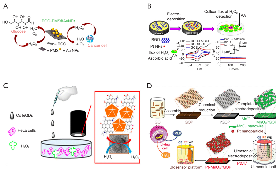
Figure 4 Electrochemical detection of H 2 O 2 based on (A) AuNPs onto mesoporous silica coated reduced graphene oxide (89); (B) reduced graphene oxide and PtNPs (83); (C) AuNPs on quantum dots (90); (D) Pt nanoparticles on freestanding reduced graphene oxide paper (rGOP) carrying MnO 2 nanowire networks (91); Reprinted with permissions from 89, 83, 90 and 91.
