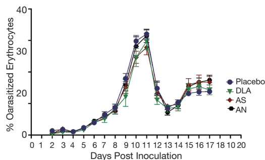
Figure 1 Babesia microti parasitemia in mice (n=6) post parasite inoculation. Drugs were administered 2 d post infection. AN, 100 mg/kg artemisinin (=167 mg/kg of powdered DLA); DLA, 100 mg/kg of DLA-delivered AN; AS, artesunate 100 mg/kg; placebo is an untreated control fed only mouse chow in a water slurry.
