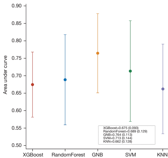
Figure 5 Forest plot of the AUC score of five machine learning models. The GNB achieved a better AUC value (0.764±0.113) in contrast to the other models. AUC, area under curve; XGBoost, eXtreme Gradient Boosting; GNB, Gaussian Naive Bayes; SVM, support vector machine; KNN, K-nearest neighbor.
