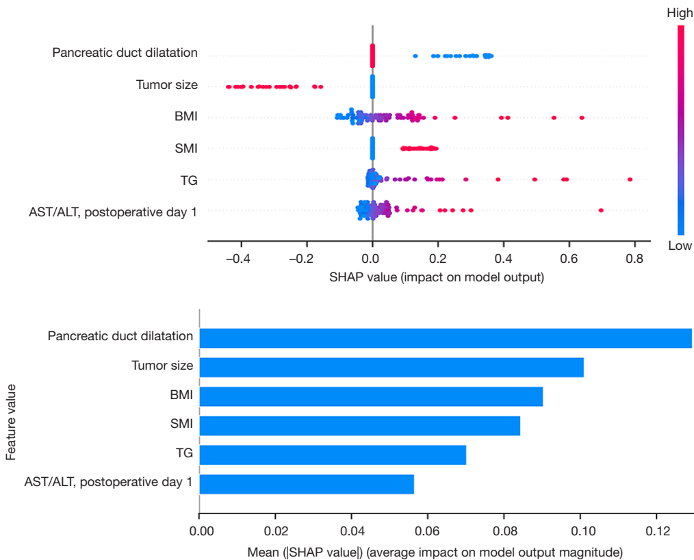
Figure 8 SHAP analysis of the Gaussian Naive Bayes model. A visualization of each sample, where each point represents a sample feature, with red representing higher values and blue representing lower values. These features were ranked according to the mean absolute value of SHAP. AST/ALT, the ratio of aspartate aminotransferase to alanine aminotransferase; BMI, body mass index; SMI, skeletal muscle index; TG, triglyceride.
