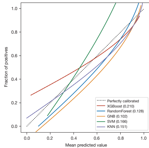
Figure 6 Calibration plots of five machine learning models. The GNB model achieved a lower Brier score (0.102) in contrast to the other models. XGBoost, eXtreme Gradient Boosting; GNB, Gaussian Naive Bayes; SVM, support vector machine; KNN, K-nearest neighbor.
