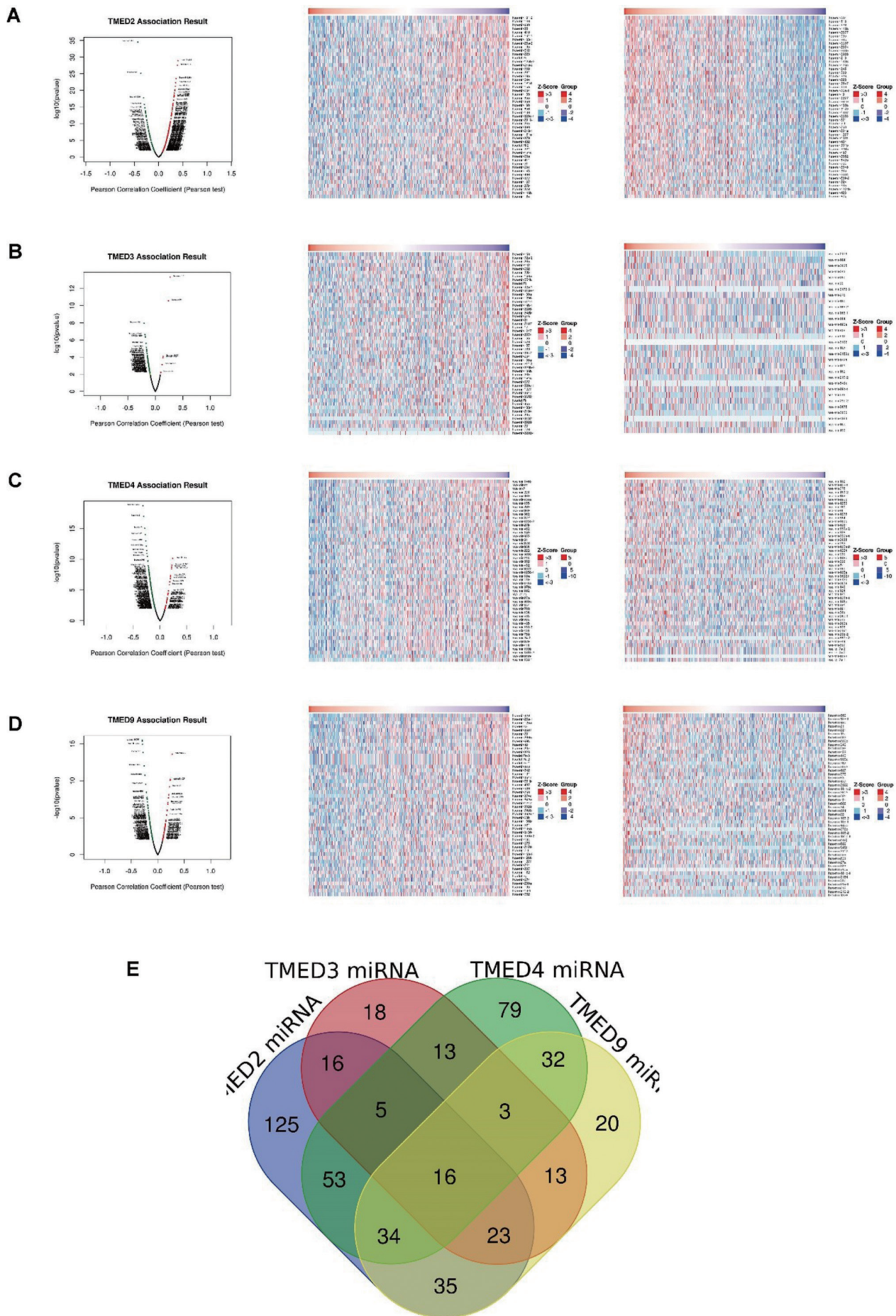
Figure S4 The correlated microRNAs of TMED2/3/4/9 in breast cancer from LinkedOmics database and their common associated microRNAs generated by Venn diagram. (A) Volcano plot of TMED2 associated microRNAs and the heatmaps for the negatively correlated significant microRNAs and positively correlated significant microRNAs. (B) Volcano plot of TMED3 associated microRNAs and the heatmaps for the negatively correlated significant microRNAs and positively correlated significant microRNAs. (C) Volcano plot of TMED4 associated microRNAs and the heatmaps for the negatively correlated significant microRNAs and positively correlated significant microRNAs. (D) Volcano plot of TMED9 associated microRNAs and the heatmaps for the negatively correlated significant microRNAs and positively correlated significant microRNAs. (E) The overlap of TMED2/3/4/9 associated microRNAs from LinkedOmics database.
