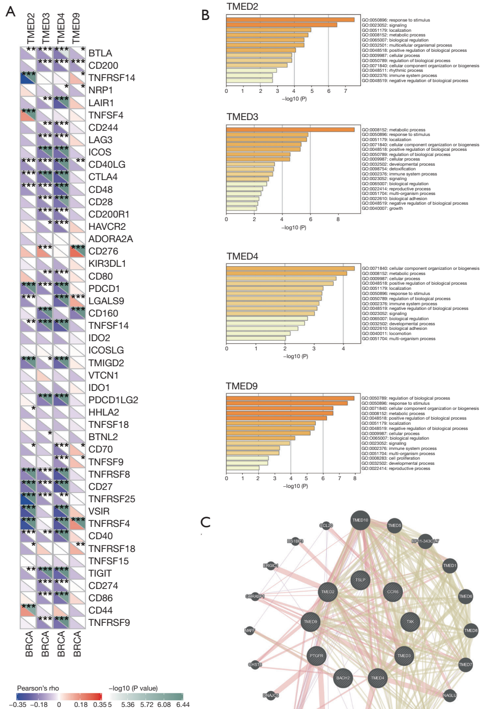
Figure 5 High expression of TMED2/3/4/9 indicated the immune-suppressive status in breast cancer. (A) Analysis of the relationship between the expressions of immune checkpoint genes and TMED2/3/4/9 mRNA levels was performed by the Sangerbox webtool. (B) GO enrichment analysis of the top 200 co-expressed genes of TMED2/3/4/9 generated by Metascape. (C) The interactome network of TMED2/3/4/9 and their common immune-related genes predicted by GeneMANIA database. *, P < 0.05 ; **, P < 0.01 ; ***, P < 0.001 . TMED, transmembrane p24 trafficking protein; BRCA, breast carcinoma; mRNA, messenger RNA; GO, Gene Ontology.
