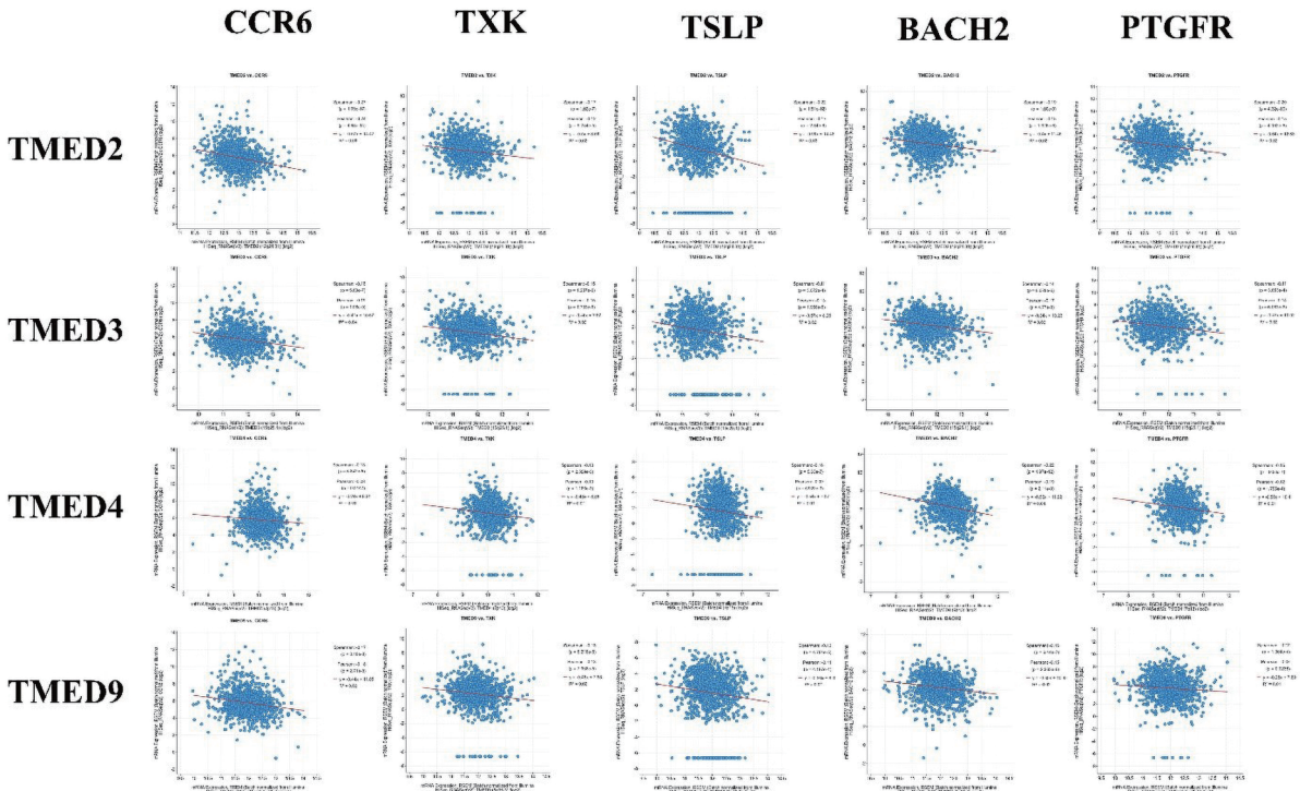
Figure S3 The prognostic value of filtered TMED2/3/4/9 immune related co-expressed genes and their correlations with TMED2/3/4/9 (A) The significant survival data of CCR6(GPR29), TXK, TSLP, BACH2, and PTGFR in breast cancer analyzed by the KM-plotter database. (B) The correlations between TMED2/3/4/9 and their common co-expressed immune-related genes. TMED2/3/4/9 was inversely correlated to the screened common immune related genes which had been screen by the combined analysis of Omcomine, Ualcan and KM-plotter.
