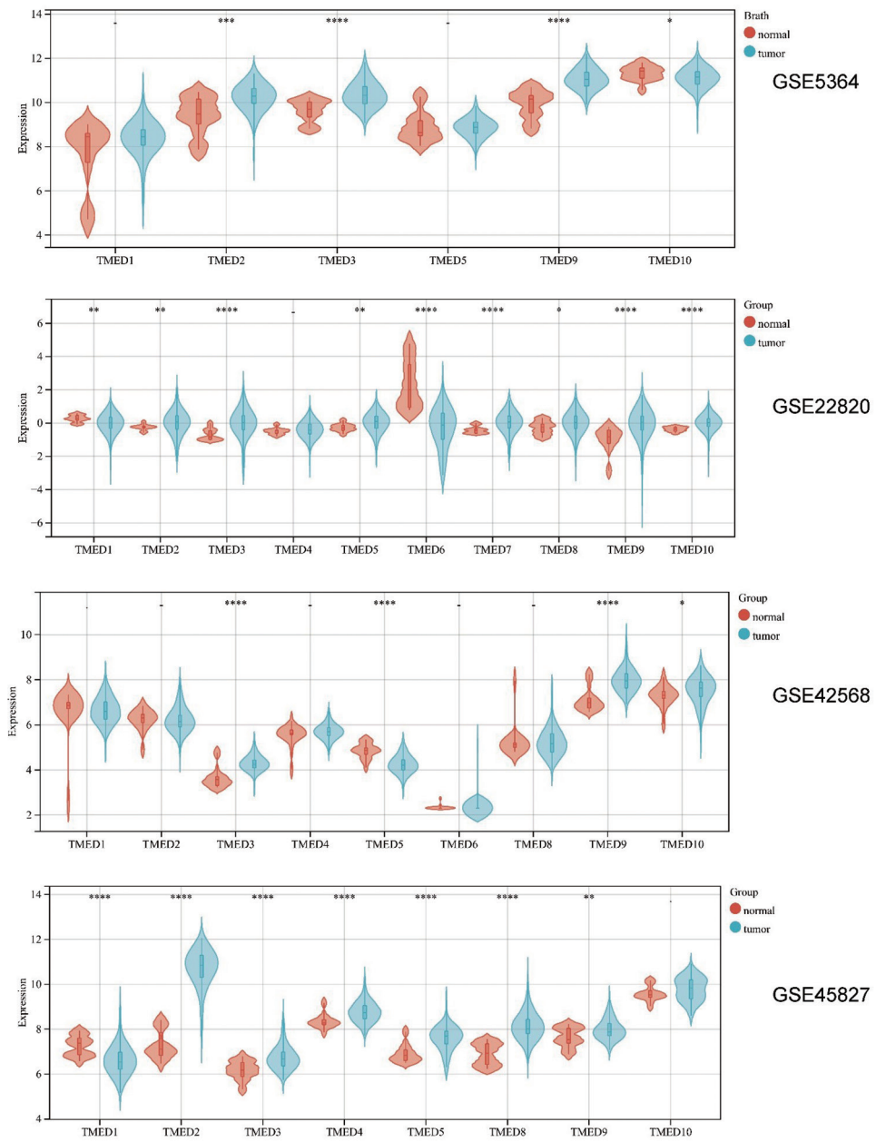
Figure S1 Expressions of TMED family in GEO microarray datasets GSE5364, GSE22820, GSE42568, GSE45827. *, P < 0.05 ; **, P < 0.01 ; ***, P < 0.001 , ****, P < 0.0001 .
