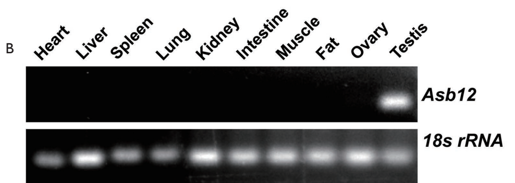
Figure S2 Asb12 is an evolutionarily conserved and testis-enriched gene among species. (A) Sequence alignment of ASB12 proteins among species. (B) RT-qPCR of Asb12 in multiple murine tissues. Asb12, ankyrin repeat and SOCS box 12.
