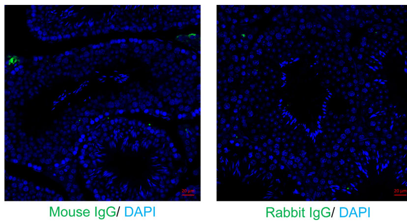
Figure S1 Representative images of mouse and rabbit IgG immunostaining in mouse testes. IgG was used as a negative control. Scale bar: 20 \mu\text{m} . DAPI, 4',6-diamidino-2-phenylindole.
