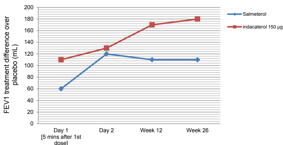
Figure 2 Differences between active treatment (salmeterol and indacaterol) over placebo for trough forced expiratory volume in 1s (FEV1). Data are presented as least squares means. Patient numbers analysed at day 2, week 12 and week 26, respectively, were 317, 320, and 300 (indacaterol), 320, 317 and 291 (salmeterol) and 321, 316, and 274 (placebo). Pre-specified 120 mL clinically important difference versus placebo. P < 0.001 versus placebo. P < 0.001 for indacaterol versus salmeterol (23).
