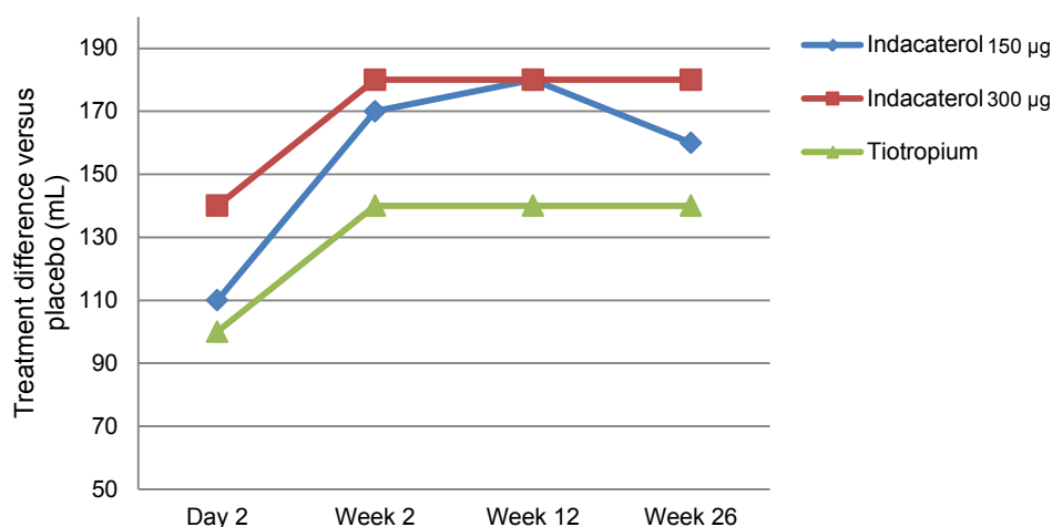
Figure 1 Differences between active treatments compared to placebo (mL) on trough forced expiratory volume in 1s (FEV1). Data are presented as least squares means. All treatment differences versus placebo were significant for superiority at P < 0.001 . Both indacaterol doses were significant for noninferiority versus tiotropium at P < 0.001 (20).
