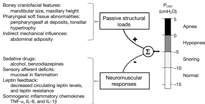
Figure 7 Upper airway collapsibility is the result of the sum of passive structural loads, which increase P_{CRIT} , and neuromuscular responses, which decrease P_{CRIT} and stabilize an inherently collapsible upper airway. Increased airway collapsibility therefore requires defects in both upper airway structure, and neuromuscular responses. Alterations in bony craniofacial features (e.g., retrognathia, decreased maxillary height) and soft tissues (e.g., peripharyngeal fat deposits and tonsillar hypertrophy) may account for structural loads. Defects in neuromuscular responses may arise from sedative drugs, sensory afferent deficits, alterations in leptin levels and/or leptin responses, or somnogenic inflammatory chemokines that may be related to obesity. Adapted from Patil et al. 2007 (48).
