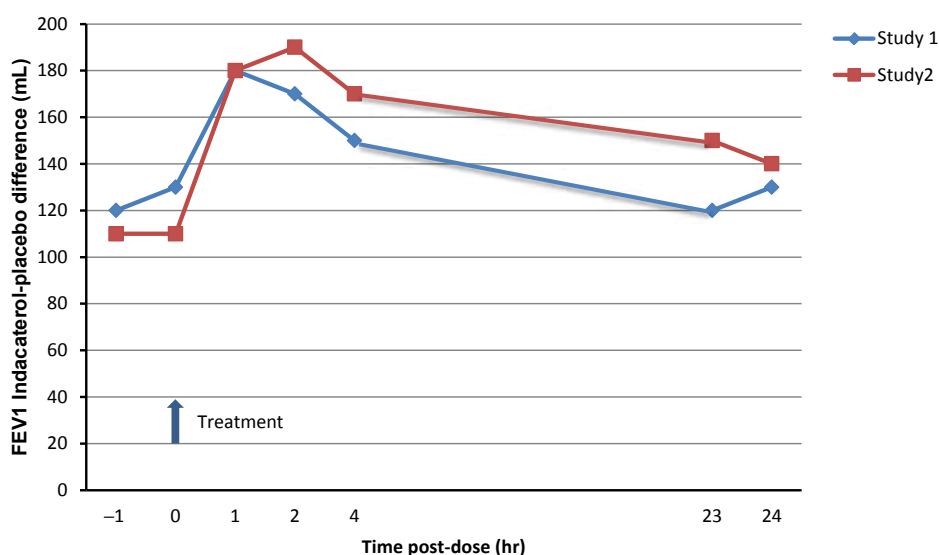
Figure 4 Indacaterol-placebo difference in forced expiratory volume in the first second of respiration (FEV1) at post-dose time points (1, 2, 4 hrs, 23 hrs 10 min, and 23 hrs 45 min) at week 12. Data represents least square means. All indacaterol-placebo differences were significant at P < 0.001 (29).
