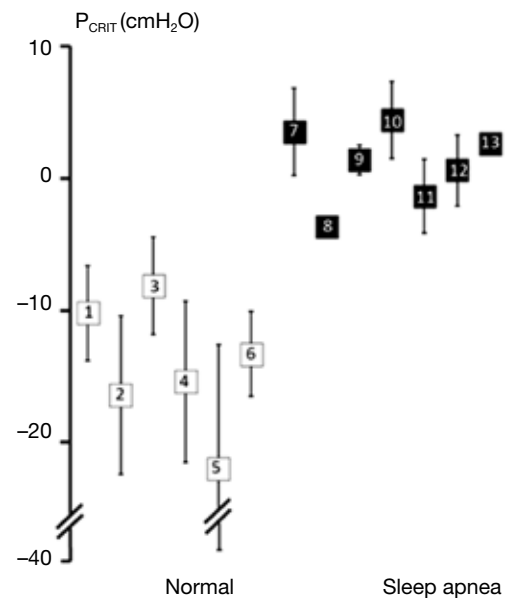
Figure 4 Summary of studies examining upper airway collapsibility (critical closing pressure, P_{CRIT} ) in normal individuals and obstructive sleep apnea (OSA) patients. Mean P_{CRIT} ( \pm standard deviation) in non-apneic controls (open squares) and apneic subjects (closed squares) are plotted. P_{CRIT} is elevated in sleep apnea patients compared to normal controls. Furthermore, these studies demonstrate minimal overlap of P_{CRIT} between disease and health, suggesting that an elevated P_{CRIT} is both sensitive and specific for OSA. Source studies, as indicated by enclosed numbers, are: 1. Meurice et al. , 1996 (37); 2. Meurice et al. , 1996 (36); 3. Issa & Sullivan, 1984 (30); 4. Gold et al. , 2002 (33); 5. Philip-Joet et al. , 1996 (38); 6. Schwartz et al. , 1988 (27); 7. Smith et al. , 1988 (28); 8. Ng et al. , 2003 (39); 9. Kirkness et al. , 2003 (34); 10. Farre et al. , 2003 (40); 11. Series et al. , 1996 (42); 12. Gold et al. , 2002 (33); 13. Sforza et al. , 2000 (32); 14. Sforza et al. , 1999 (31); 15. Issa & Sullivan, 1984 (30). Adapted from Pack, 2009 (41).
