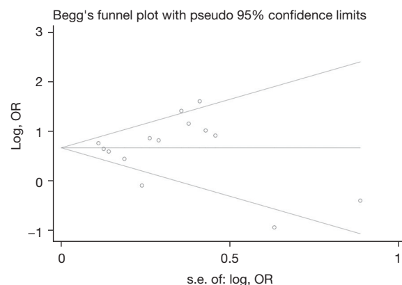
Figure 4 Funnel plot with 95% confidence interval.
