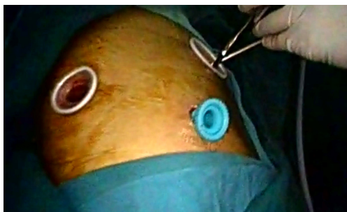
Figure 1 Trocars position.
