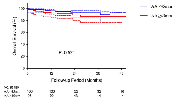
Figure S1 Kaplan-Meier curves for overall survival in patients with AA \geq 45 and < 45 mm ( P=0.521 ). AA, ascending aorta.
