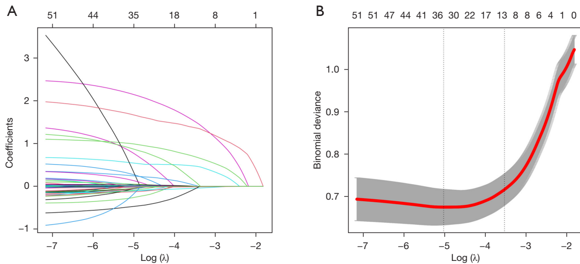
Figure 2 The LASSO regression was used to extract features. (A) The results revealed that 38 variables were retained at the point where the error was minimized, which is represented by the position of the dotted line on the left (B). To prevent overfitting and simplicity of the model, only variables within one standard error (1se) of the minimum error were selected, and 12 variables were retained, represented by the location on the dotted line on the right (B). LASSO, least absolute shrinkage and selection operator.
