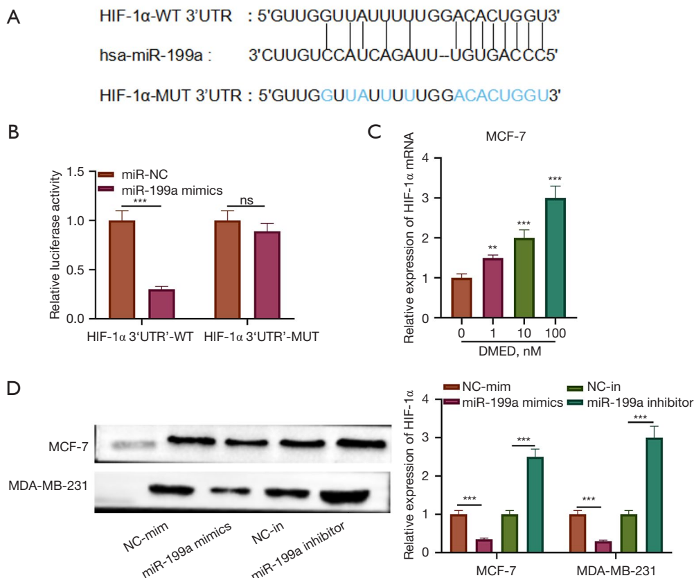
Figure 4 MiR-199a targeting HIF-1α. (A) Bioinformatics website shows that HIF-1α contains miR-199a binding site. (B) Double luciferase assay was used to detect the binding of miR-199a and HIF-1α. (C) The level of HIF-1α mRNA was detected using QRT-PCR. (D) The level of HIF-1α was detected using western blot. **, P<0.01; ***, P<0.001. QRT-PCR, quantitative real-time polymerase chain reaction.
