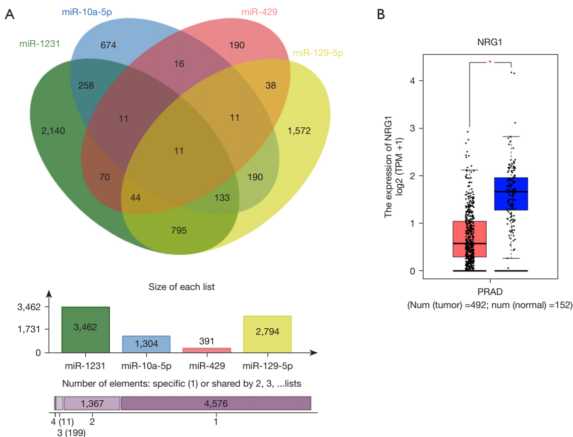
Figure 4 Target gene prediction and genes differentially expressed in GEPIA. (A) Target genes of the four-miRNA panel predicted from miRWalk 3.0. (B) Under the criterion of P value <0.01 and |\log_2\text{foldchange}| cutoff >1 based on the expression level, expression levels of NRG1 were significantly dysregulated in 492 prostate cancer patients and 152 normal controls. *, P<0.05. PRAD, prostate adenocarcinoma; TPM, transcripts per million; GEPIA, Gene Expression Profiling Interactive Analysis.
