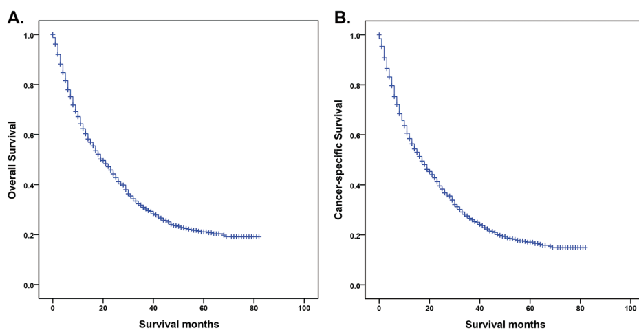
Figure S2 Kaplan-Meier curve estimate the overall survival and cancer-specific survival of lung metastatic RCC. (A) Overall survival; (B) cancer-specific survival.
