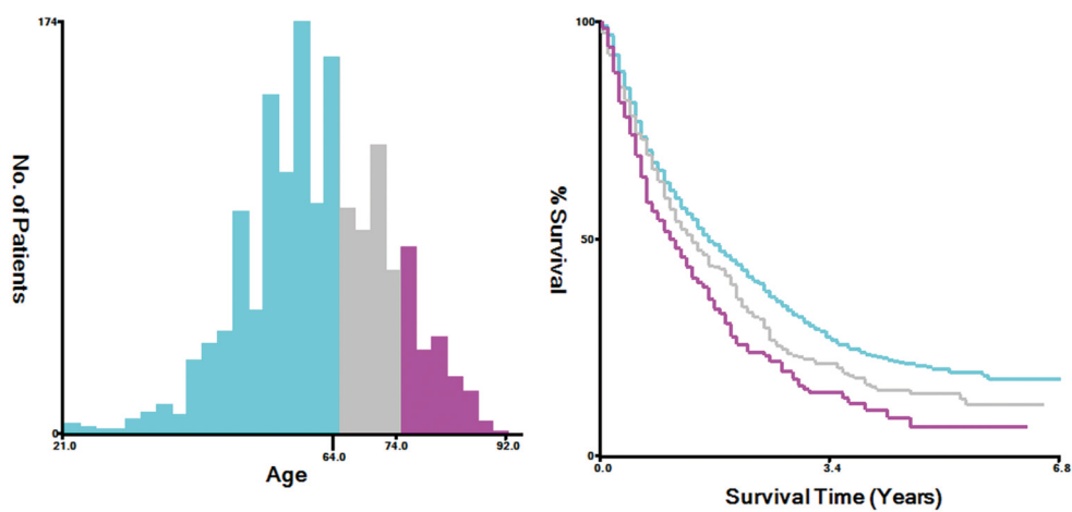
Figure S1 Using X-tile software to group the age of patients with lung metastatic RCC.
