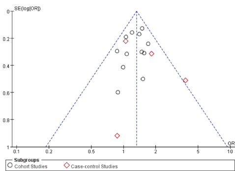
Figure S1 Funnel plots for the indexes (Female).
