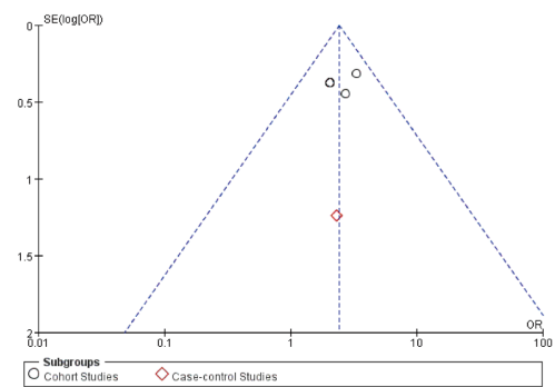
Figure S2 Funnel plots for the indexes (lymphatic metastasis larger than 6).
