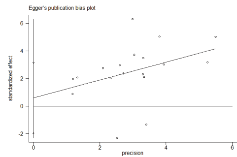
Figure S4 Egger's publication bias plot (adenocarcinoma).
