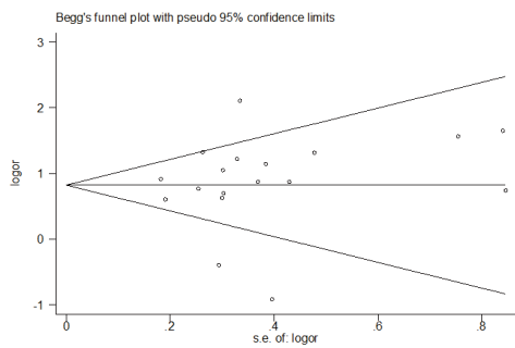
Figure S5 Begg's funnel plot (adenocarcinoma).
