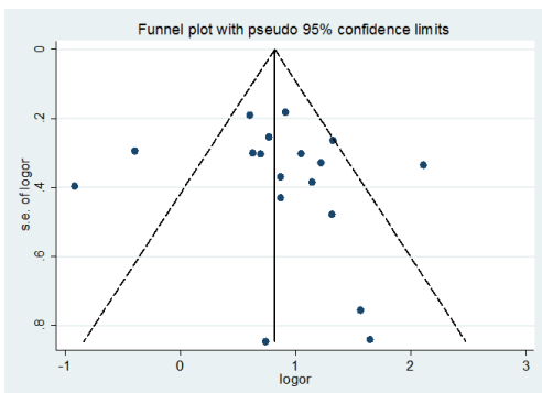
Figure S3 Funnel plots for the indexes (adenocarcinoma).
