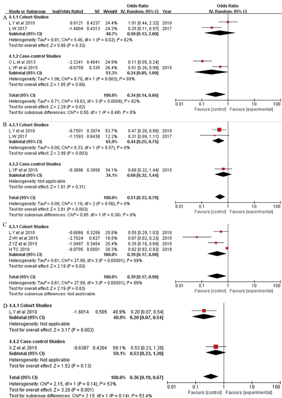
Figure S6 Meta-analysis of survival rates. (A) 1-year survival rate; (B) 2-year survival rate; (C) 3-year survival rate; (D) 5-year survival rate.
