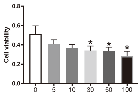
Figure S1 Viability of A549 cells exposed to BALF. *, P < 0.05 vs. the control group. BALF, bronchoalveolar lavage fluid.
