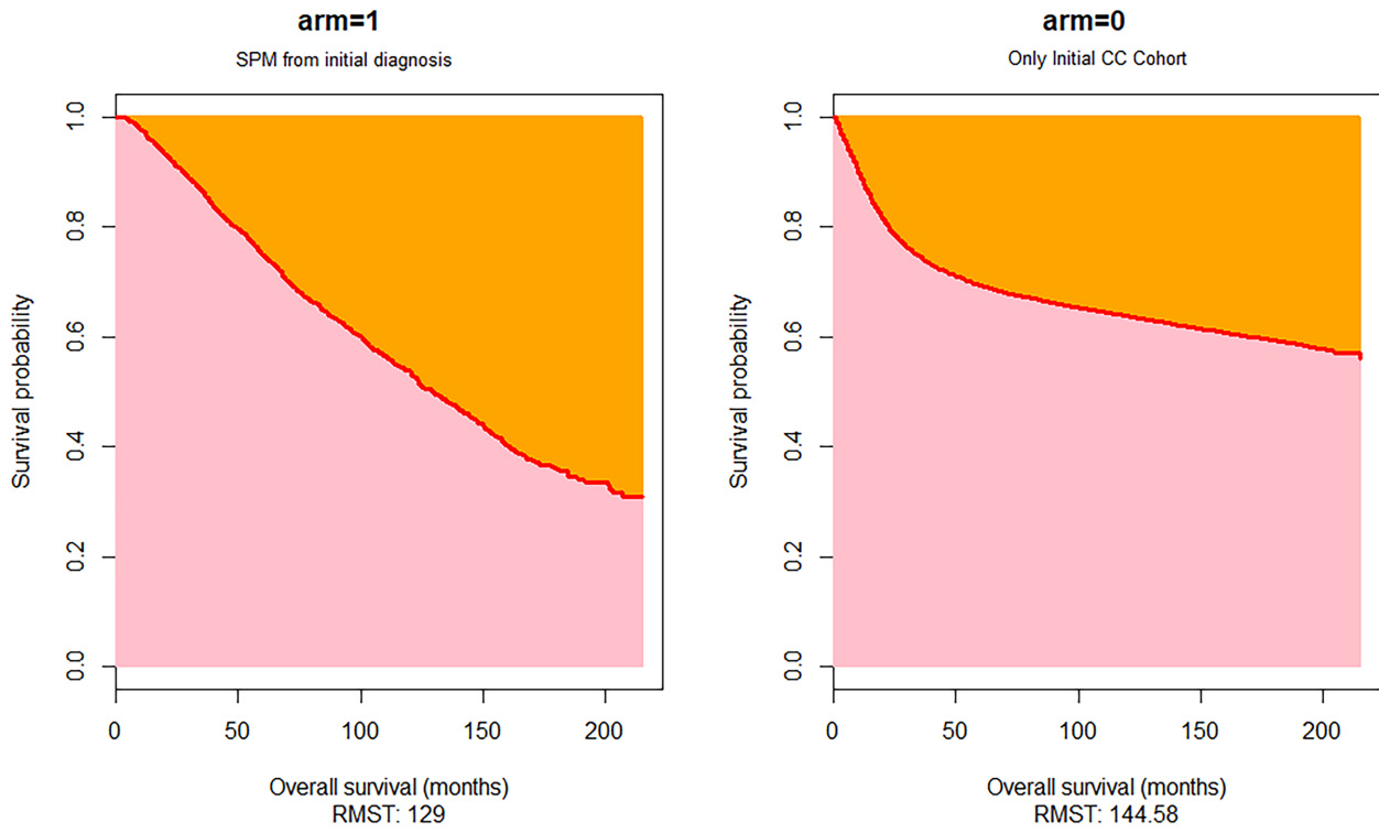
Figure S2 Restricted mean survival time (RMST) of CC patients with and without SPM.
