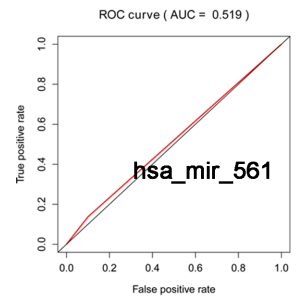
Figure S1 The AUC of miRNA model was higher than that of every single miRNA or TNM stage. AUC, area under curve.
