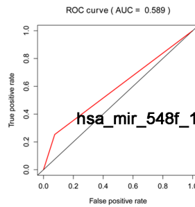
Figure S1 The AUC of miRNA model was higher than that of every single miRNA or TNM stage. AUC, area under curve.
