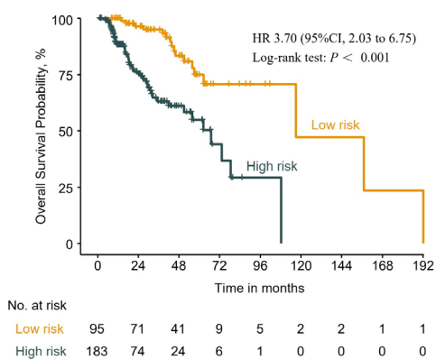
Figure S1 The OS of the validation cohort was divided into two significant different groups by the cutoff.
