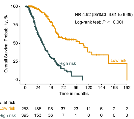
Figure S2 The OS of the combination cohort was divided into two significant different groups by the cutoff.
