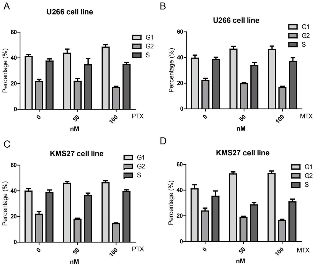
Figure S1 Effects of PTX and MTX on the cell cycles of MM cell lines. (A) Effects of PTX on the cell cycle of the U266 cell line; (B) effects of MTX on the cell cycle of the U266 cell line; (C) effects of PTX on the cell cycle of the KMS27 cell line; (D) effects of MTX on the cell cycle of the KMS27 cell line. PTX, pralatrexate; MTX, methotrexate; MM, multiple myeloma.
