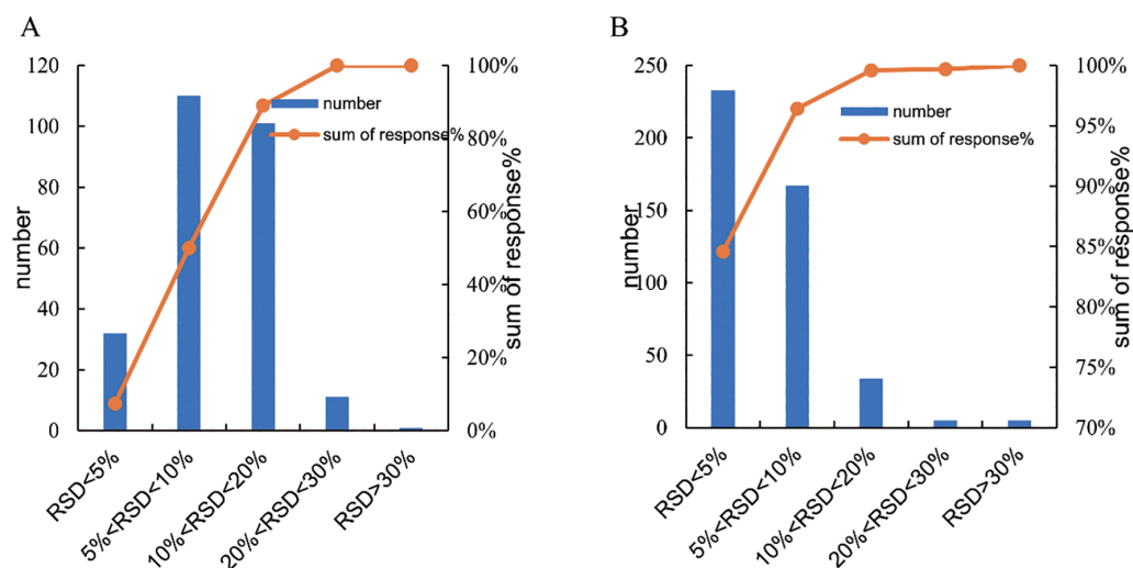
Figure S1 CV distribution of all detected metabolites and lipids in 11 QCs. Number %, percentage of number of lipids within a defined range of CV value. Sum of response %, percentage of total response of lipids below a special criteria of CV value. (A) Metabolomics; (B) lipidomics. CV, coefficient of variation; QCs, quality control samples; RSD, relative standard deviation.
