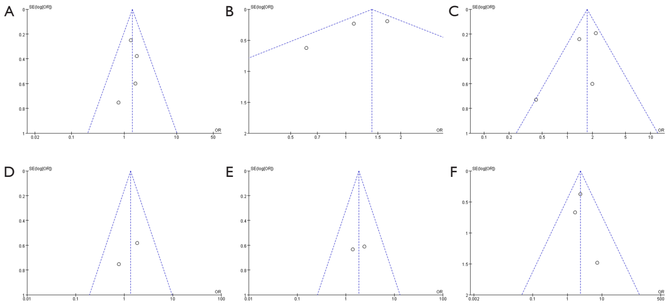
Figure S1 The funnel plot of 1-, 3-, 5-year pooled overall survival rate (A-C); The funnel plot of 1-, 5-year pooled recurrence-free survival rate (D,E); R0 resection rate (F).
