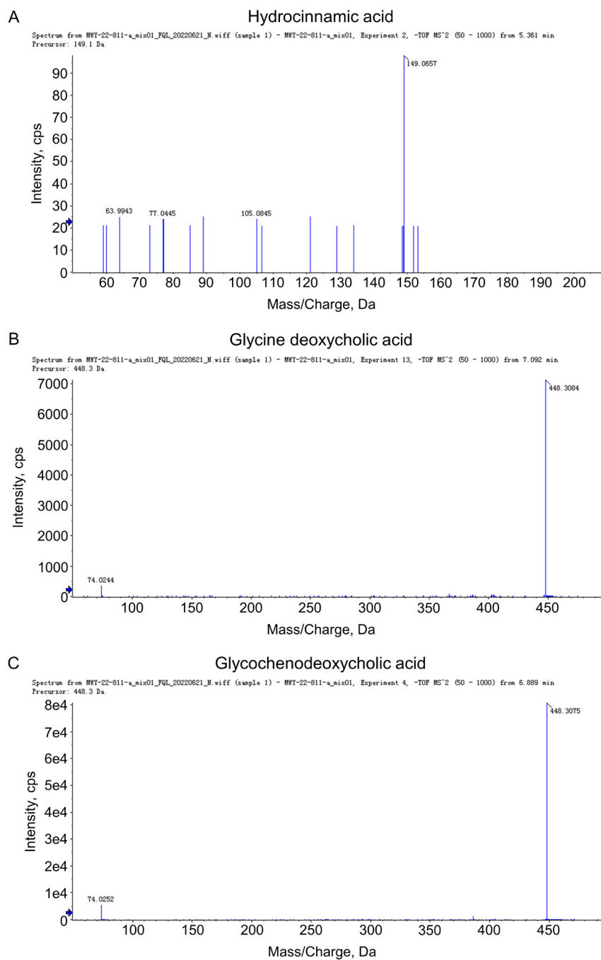
Figure S1 Mass spectrum of the hydrocinnamic acid (A), glycine deoxycholic acid (B) and glycochenodeoxycholic acid (C).
