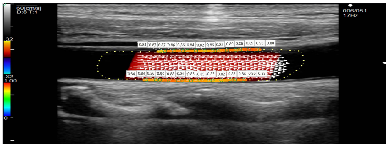
Figure S1 WSS at various points on the anterior and posterior walls of the carotid artery. WSS, wall shear stress.
