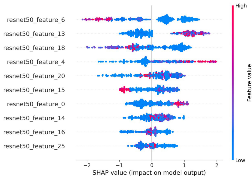
Figure S1 SHAP analysis for deep learning model.
