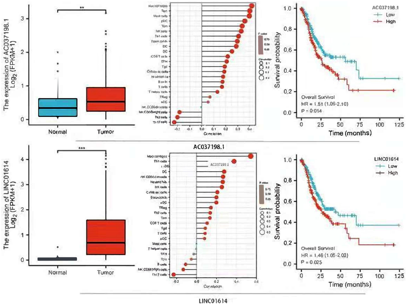
Figure S1 The expression of lncRNA used for model construction in GC and its role in tumor immunity were analyzed by difference, prognosis and immune analysis. **, P < 0.01 ; ***, P < 0.001 . GC, gastric cancer.
