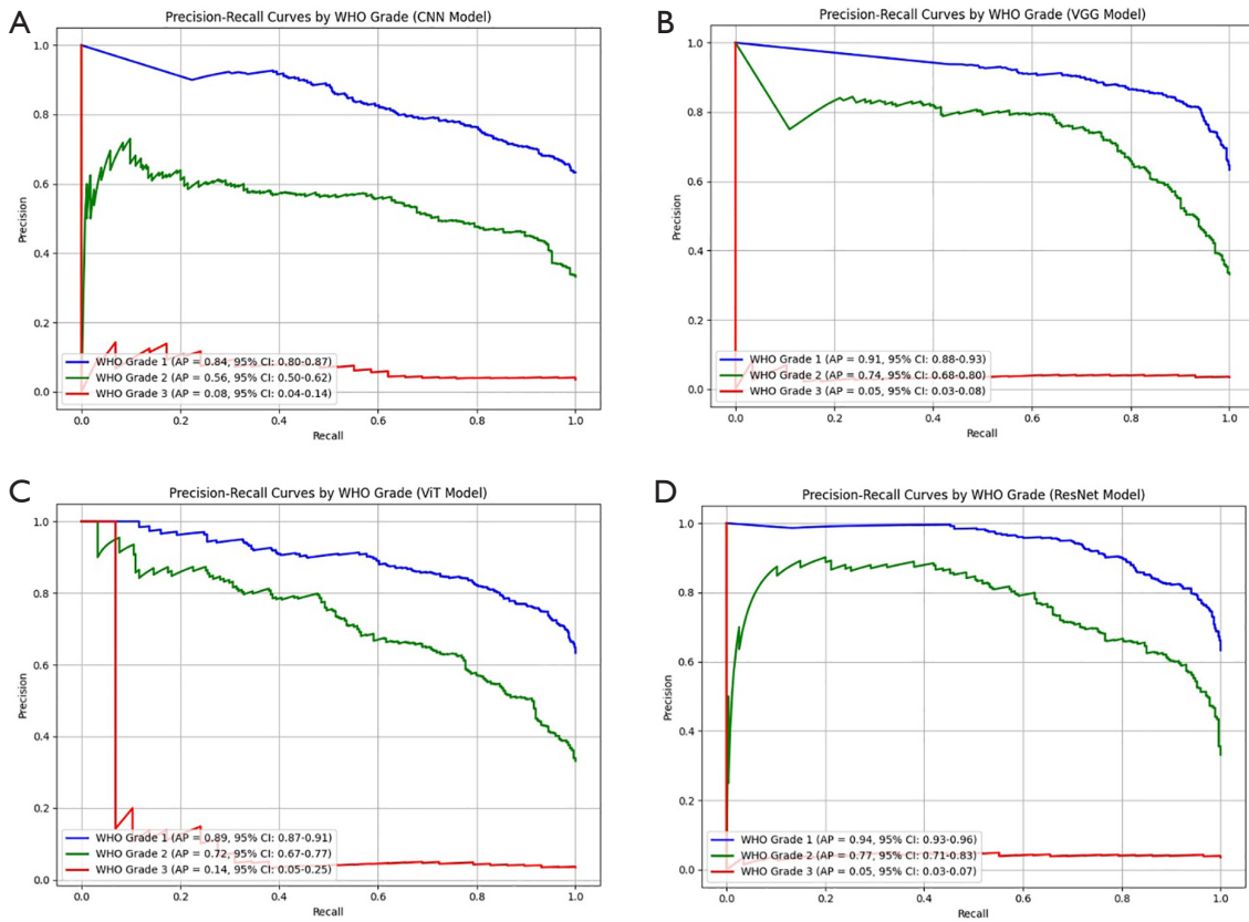
Figure S1 The Precision-Recall curves for each WHO grade using the four deep learning models: (A) CNN; (B) VGG; (C) ViT; (D) ResNet. AP, area under the precision-recall curve; CI, confidence interval; CNN, convolutional neural network; ResNet, residual neural network; VGG, visual geometry group; ViT, vision transformer; WHO, World Health Organization.
