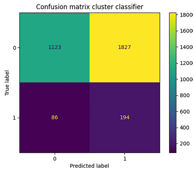
Figure S2 Confusion matrix for AHA plot classifier using cluster classification approach. AHA, American Heart Association.
