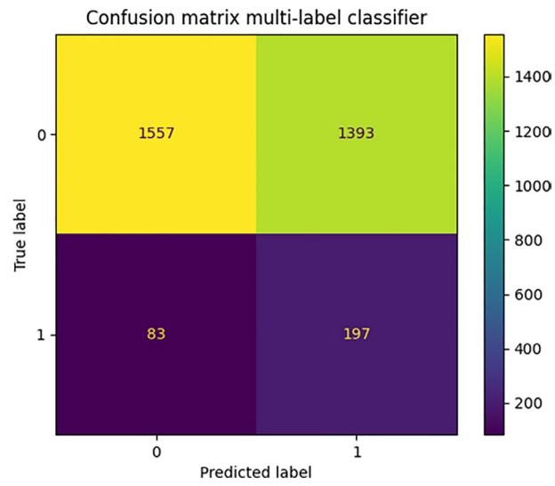
Figure S1 Confusion matrix for AHA plot classifier using multi-label classification approach. AHA, American Heart Association.
