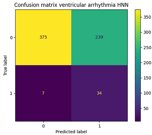
Figure S4 Confusion matrix for ventricular arrhythmia prediction model using HNN. HNN, hybrid neural network.
