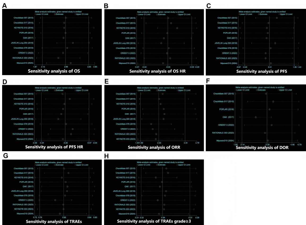
Figure S1 Sensitivity analysis of OS (A), OS HR (B), PFS (C), PFS HR (D), ORR (E), DOR (F), TRAEs(G) and TRAEs grade \geq 3 (H).
