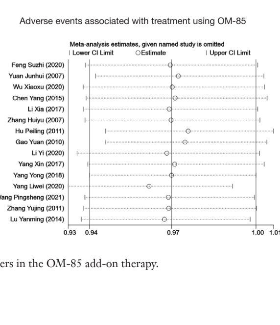
Figure S6 Sensitivity analysis of parameters in the OM-85 add-on therapy.
