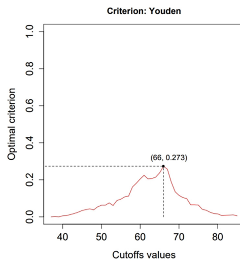
Figure S2 The best cutoff point for age.
