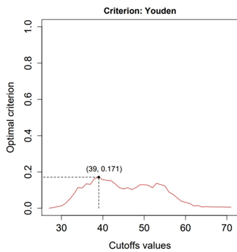
Figure S1 The best cutoff point for left atrial diameter.
