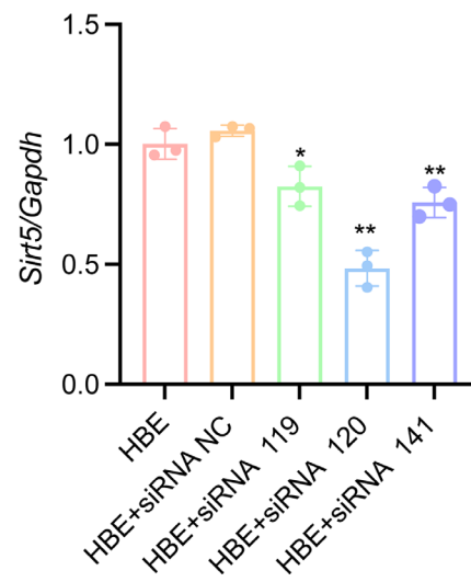
Figure S1 Screening of optimal siRNA SIRT5 sequences by qRT-PCR. *, 0.01 < P < 0.05 , vs. HBE group; **, P < 0.01 , vs. HBE group. SIRT5, Sirtuin 5; HBE, human bronchial epithelial; NC, negative control; qRT-PCR, quantitative real-time polymerase chain reaction.
