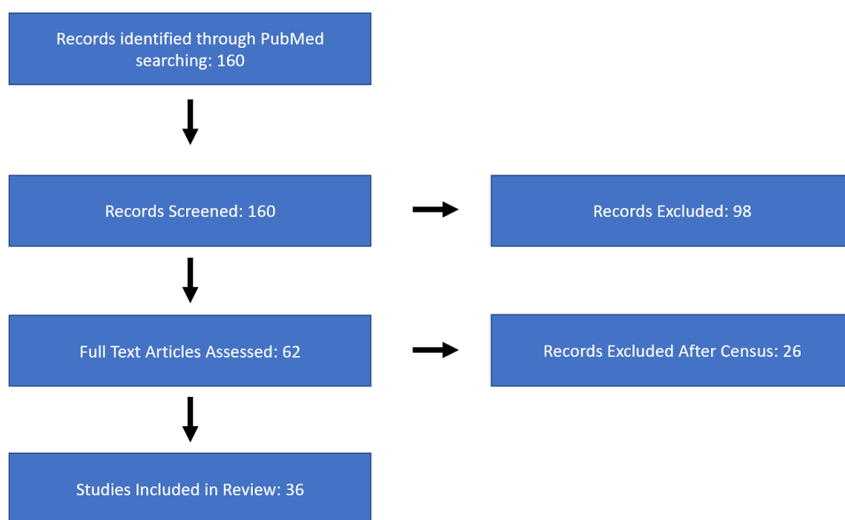
Figure S1 Flow diagram depicting our search methods.
