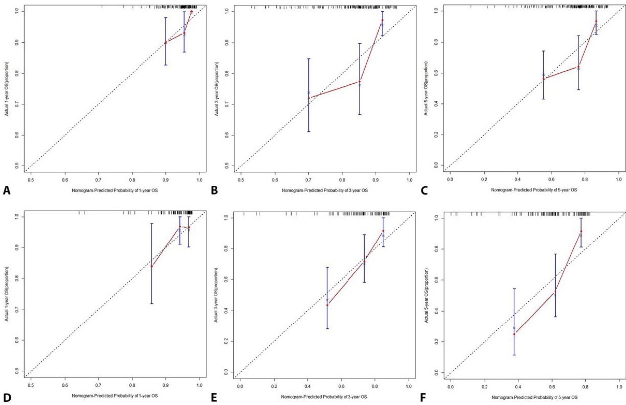
Figure S1 Calibration plots of the prediction model for individually predicting the survival in the training cohort (A, 1-year survival; B, 3-year survival; C, 5-year survival) and the external validation cohort (D, 1-year survival; E, 3-year survival; F, 5-year survival).
