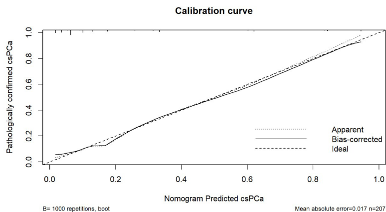
Figure S1 Calibration curves of the special nomogram for young patients suspected to prostate cancer.
