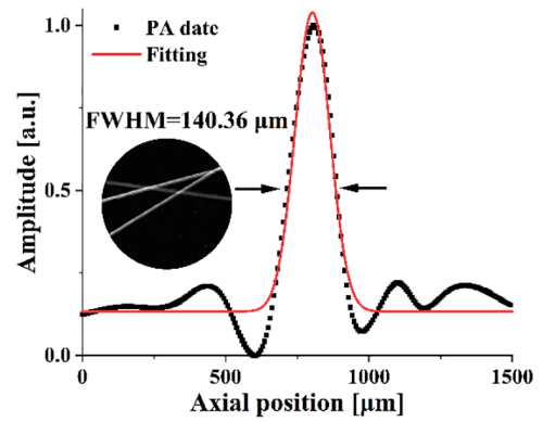
Figure S2 The axial resolution of the system evaluated with a carbon fiber. a.u., arbitrary unit; PA, photoacoustic; FWHM, full width at half-maximum.
