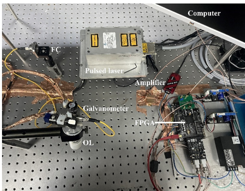
Figure S1 Photograph of the photoacoustic imaging system. FC, fiber coupler; FPGA, field-programmable gate array; OL, objective lens.
