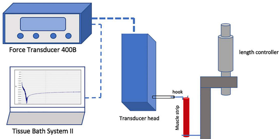
Figure S2 The muscular force transducer head and controller of 400B series of high-level output force transducers system. The muscular strip was hanged between the force sensor hook and force/length controller. Consistent 330-gram force was applied by the length controller, and the rebound force and muscular stiffness were recorded by the force sensor connected to a Myobath Tissue Bath System II.
