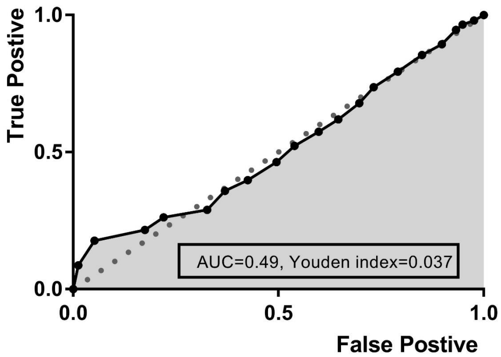
Figure S1 t-ROC curve of year of diagnosed on 5-year survival
