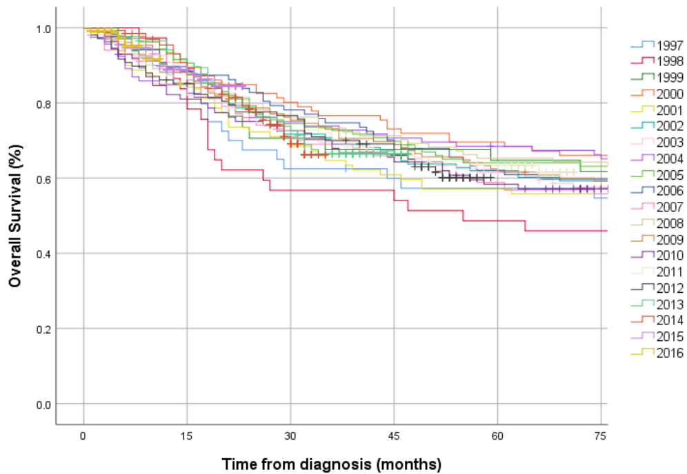
Figure S2 KM curves showed comparable surviving among diagnosed year in 1997 to 2016
