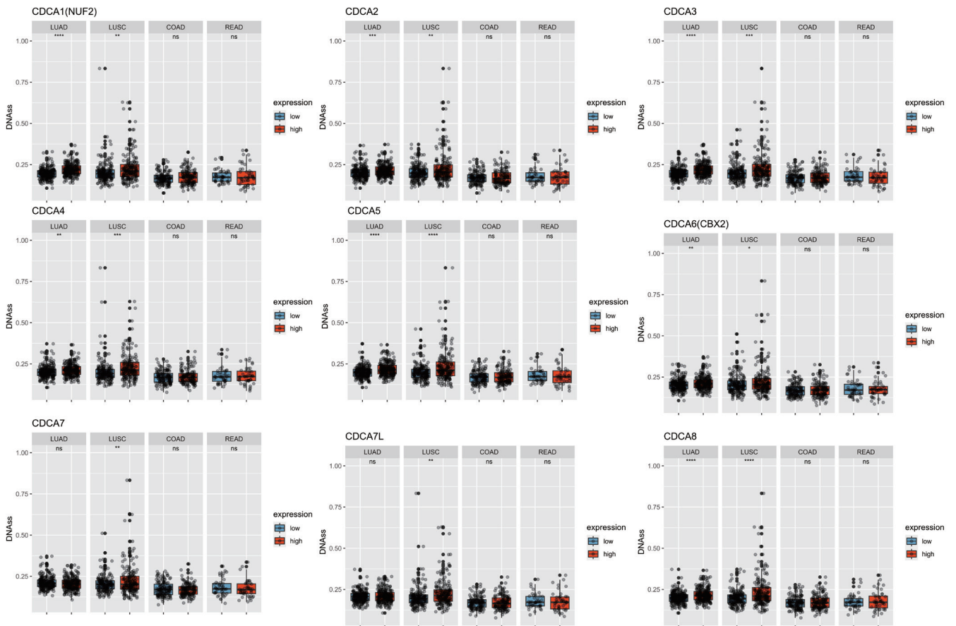
Figure S2 DNAss difference of CDCAs in lung cancer and bowel cancer. DNAss, DNA methylation-based stemness scores.
