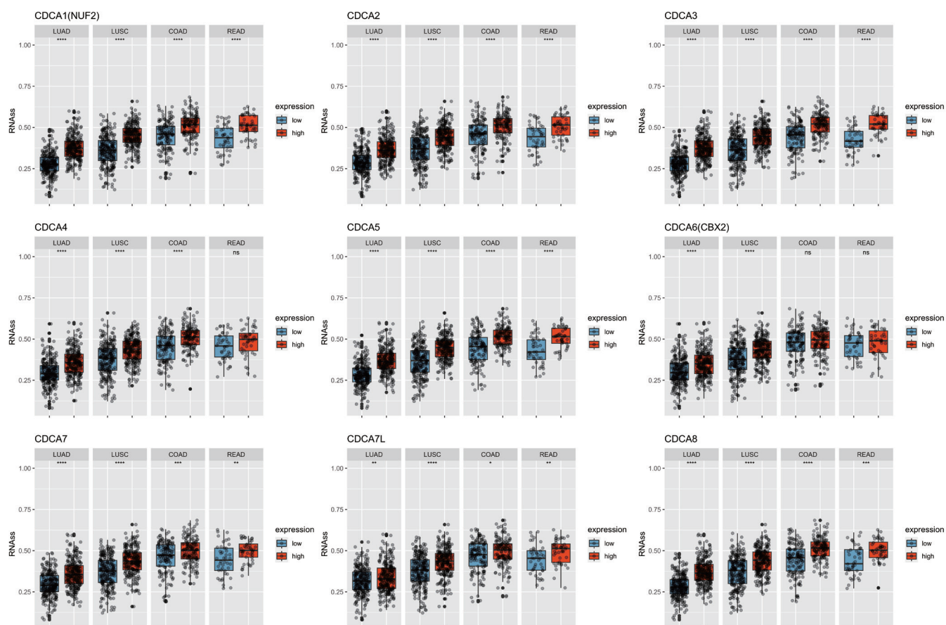
Figure S1 CDCA s differ in RNAss in lung and bowel cancer. RNAss, RNA-based stemness score.
