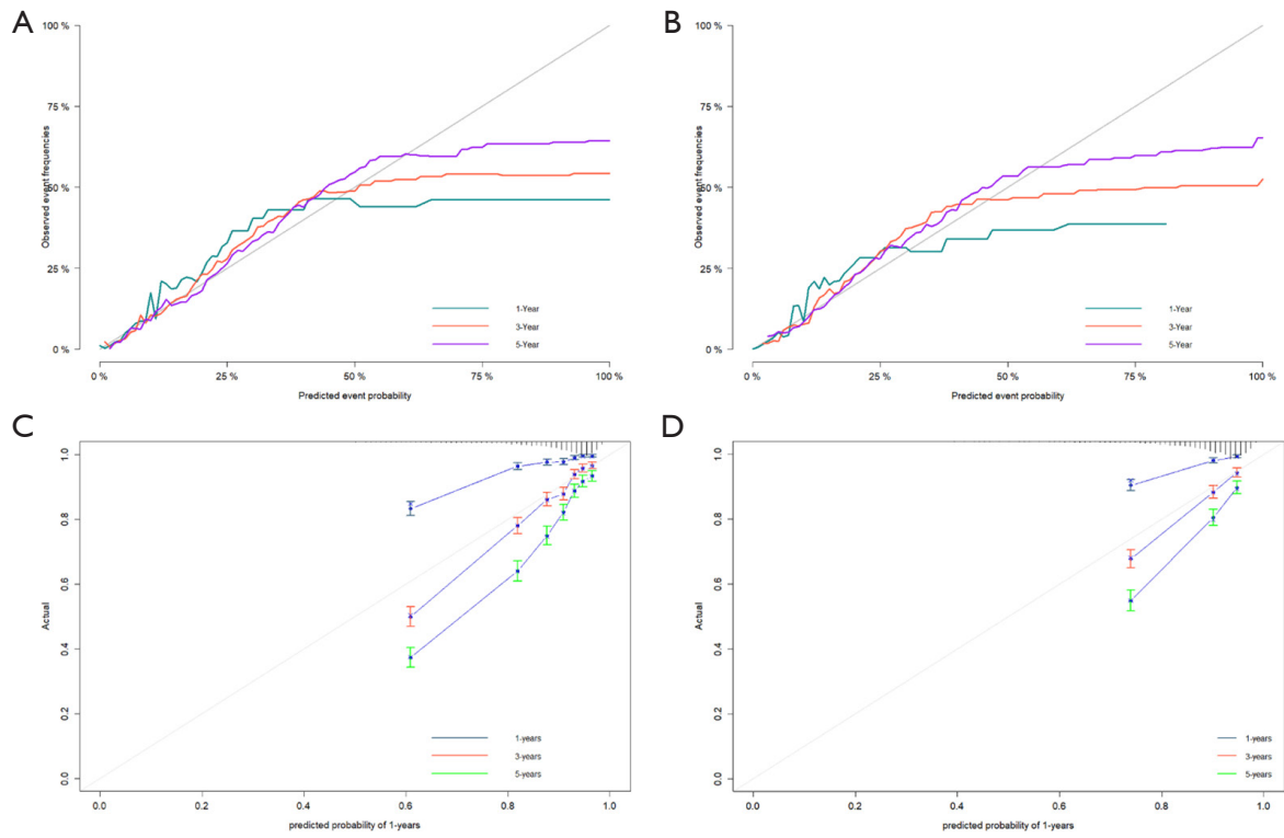
Figure S2 Calibration plots of competing risk nomograms for CSS in postmenopausal EC patients undergoing surgery combined with radiotherapy in (A) training cohort and (B) validation cohort, and calibration plots of Cox proportional hazards nomograms for (C) training cohort and (D) validation cohort.
