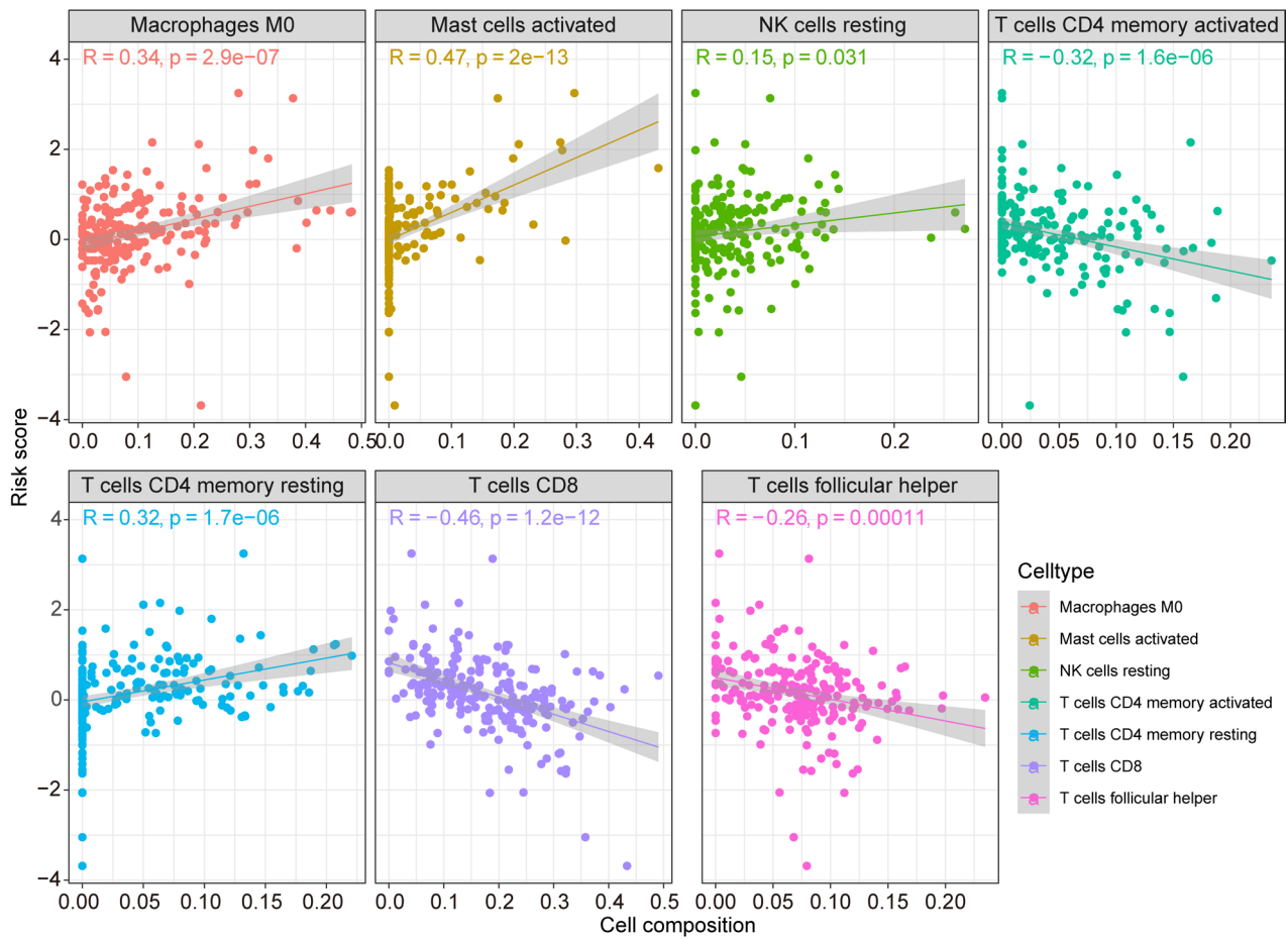
Figure S2 Correlation analysis. Correlation between RiskScore and infiltration level of CD4 memory activated T cells, CD8 T cells, follicular helper T cells, M0 macrophages, activated mast cells, resting NK cells, and CD4 memory resting T cells.
