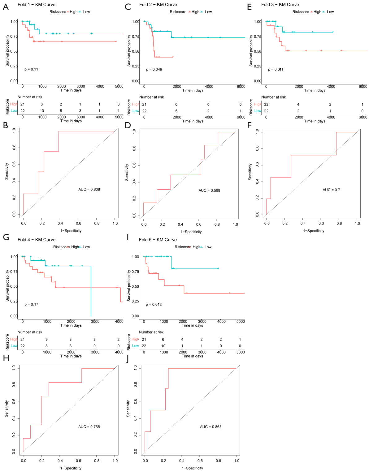
Figure S1 5-fold cross-validation. (A) KM survival curve of LRG and HRG in Fold 1. (B) ROC curve based on the data in Fold 1. (C) KM survival curve of LRG and HRG in Fold 2 (D) ROC curve based on the data in Fold 2. (E) KM survival curve of LRG and HRG in Fold 3. (F) ROC curve based on the data in Fold 3. (G) KM survival curve of LRG and HRG in Fold 4. (H) ROC curve based on the data in Fold 4. (I) KM survival curve of LRG and HRG in Fold 5. (J) ROC curve based on the data in Fold 5.
