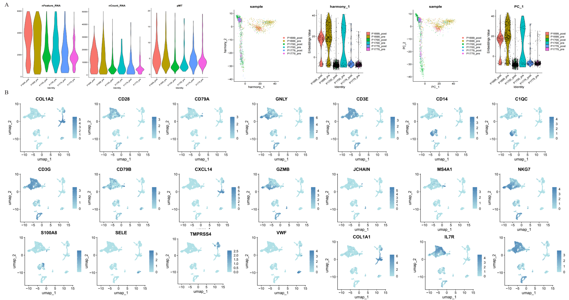
Figure S1 Clustering and dimension reduction analysis of single-cell data. (A) Quality control of the single-cell RNA sequencing dataset; (B) the expression of 21 genes in the single-cell dataset. scRNA-seq, single-cell RNA sequencing.
