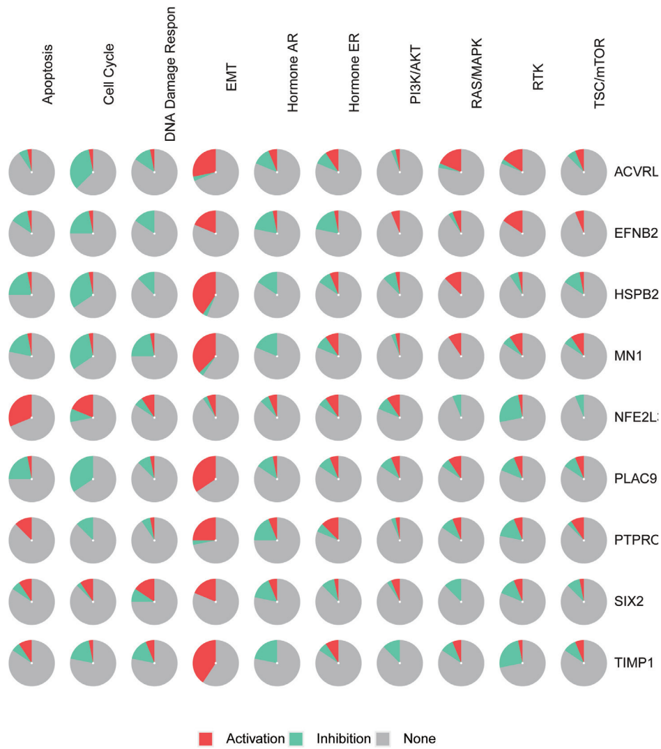
Figure S2 Analysis activation pathways of nine gene which used to construct CRS3.
