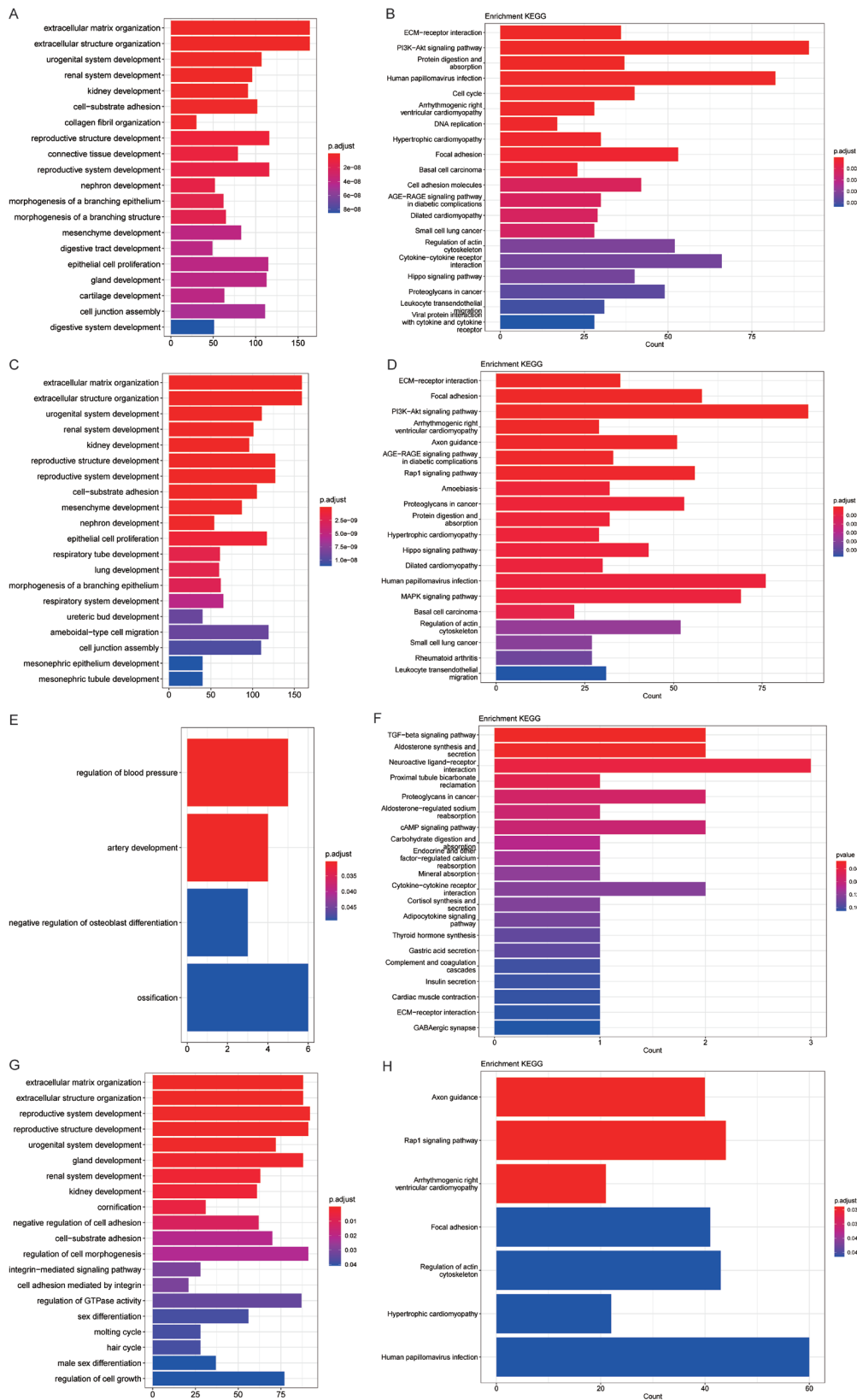
Figure S1 Functional enrichment results of SMGs in four CAFs clusters.
