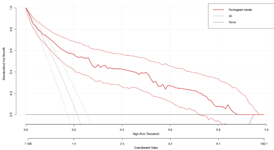
Figure S2 The DCA predicting breast cancer severity. DCA, decision curve analysis.
