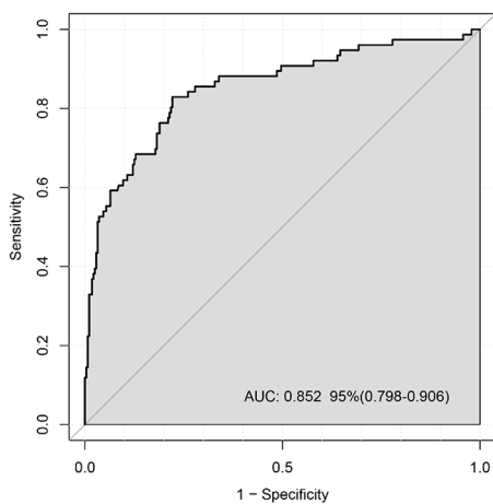
Figure S1 The receiver operating characteristic curve predicting breast cancer severity. AUC, area under the curve.
