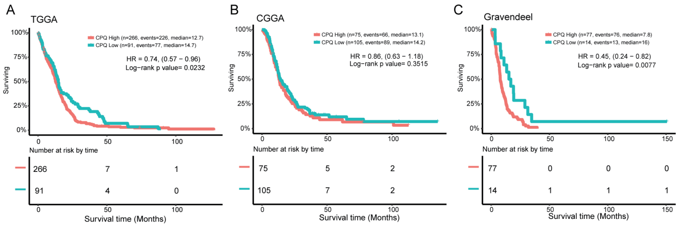
Figure S3 Kaplan-Meier analysis of CPQ expression and OS in IDH wildtype GBM populations based on TCGA-GBM (A), CGGA (B), Gravendeel (C) datasets.
